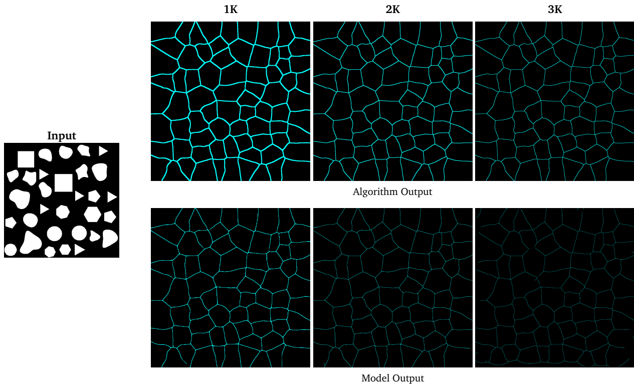
Figure 8: Qualitative comparison of algorithmic and learning-assisted Voronoi extraction across increasing grid resolutions.
