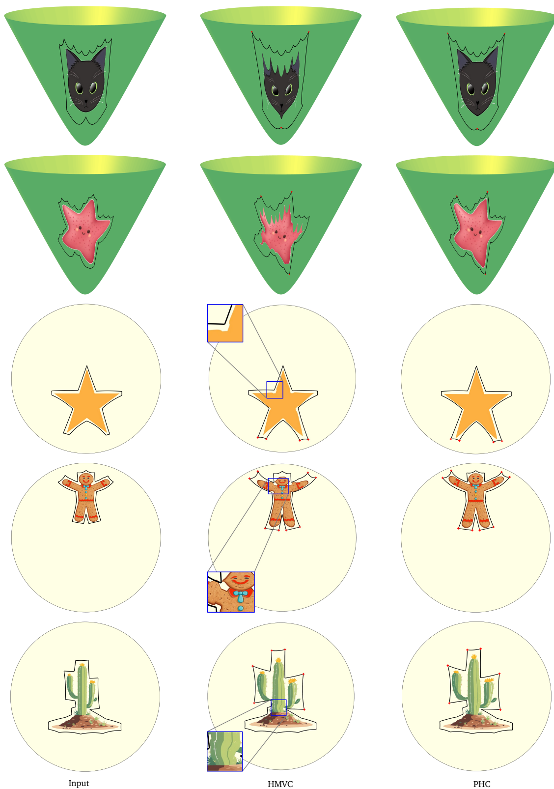
Figure 4: Comparison of image deformations using hyperbolic mean value coordinates (HMVC) and positive hyperbolic ones (PHC) on the hyperbolic plane and the Poincaré disc.
